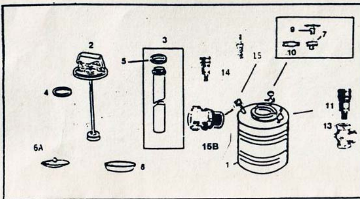
- Parts List -
